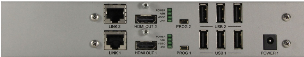
Figure 3. Sample CrystalView EX HDMI Dual Receiver Rear Panel
