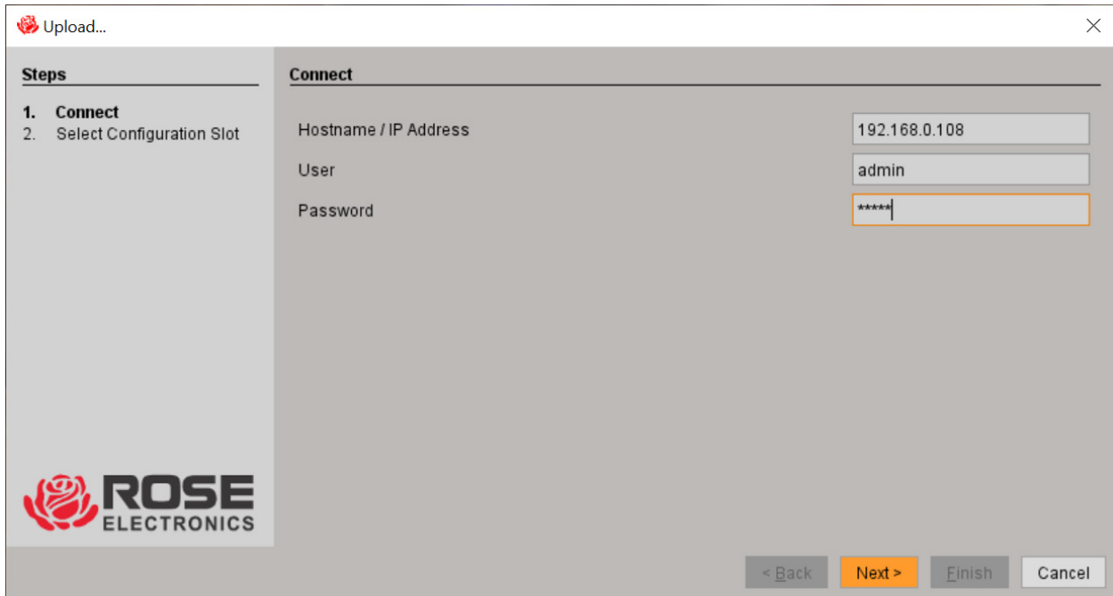
Figure 143. Saving Configuration to Internal Storage with the Java Tool
