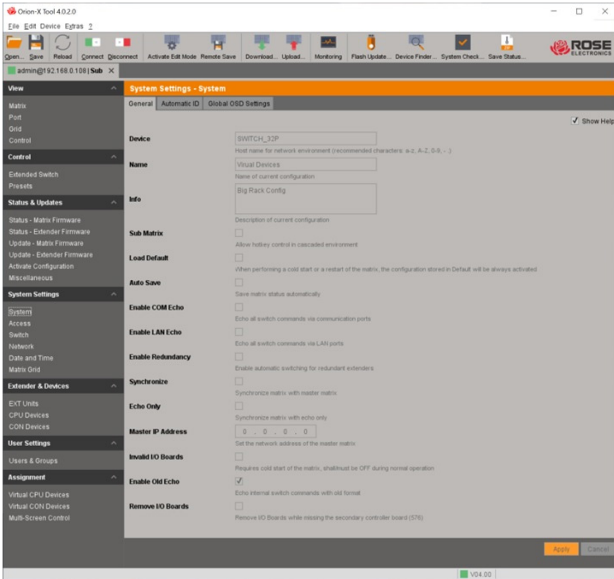
Figure 54. System Settings – System Screen in the Java Tool
