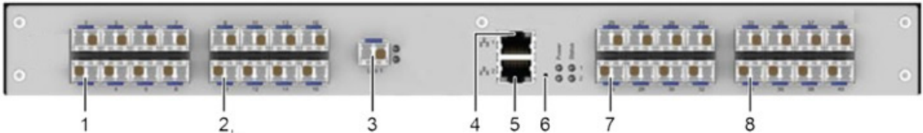
Figure 13. Front Panel, 32-Port Model with Grid Port and all Fiber Ports
