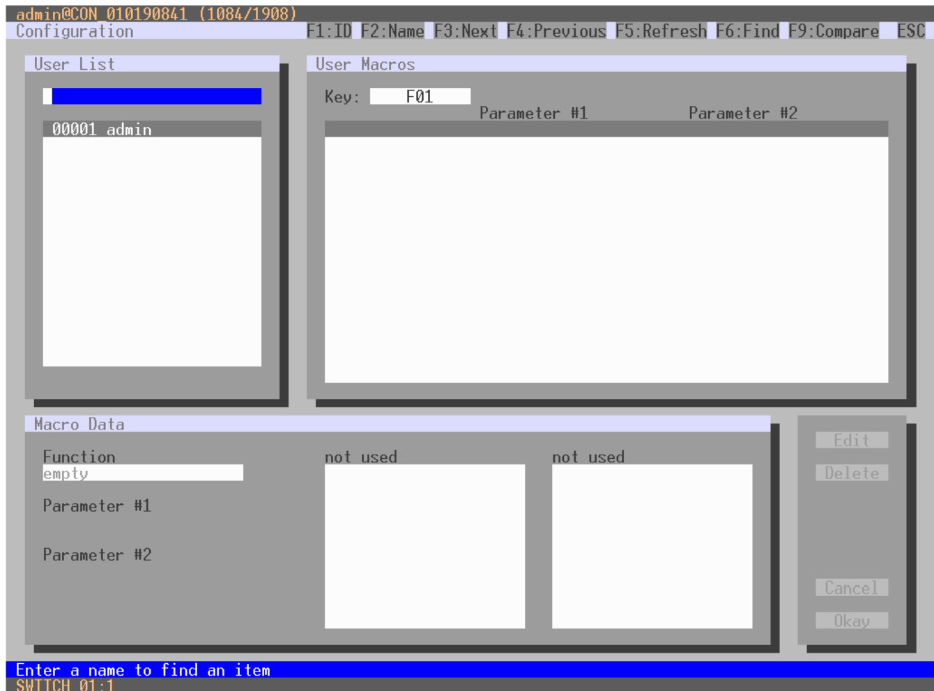
Figure 95. Setting Up User Macros through the OSD
