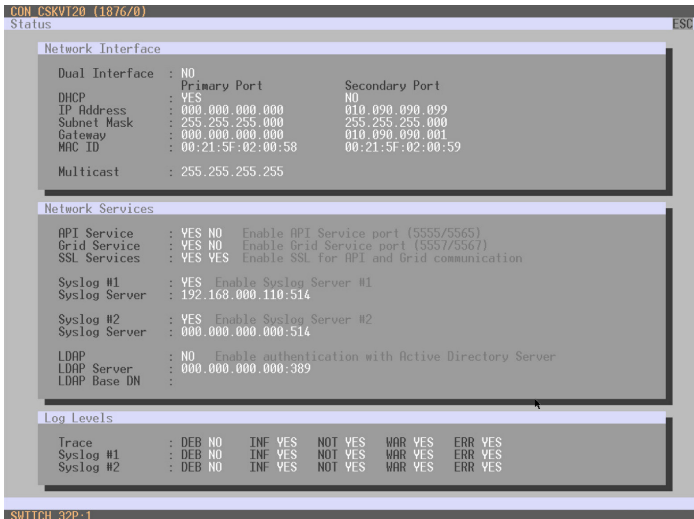
Figure 204. Network Status in the OSD
