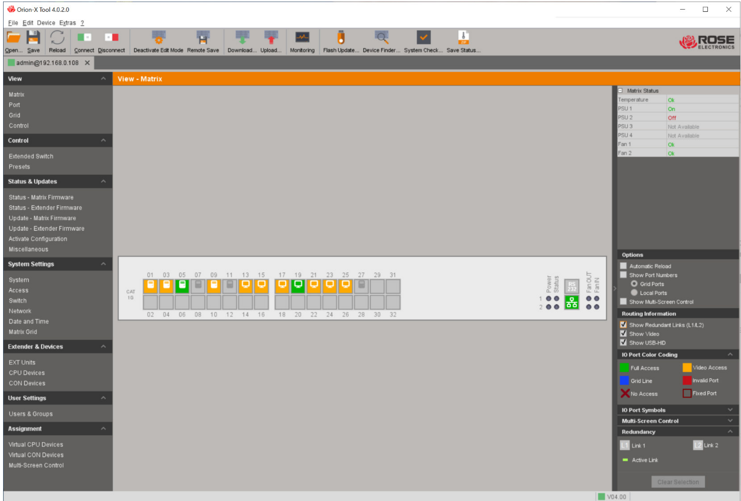
Figure 193. Checking Redundant Links with the Java Tool
