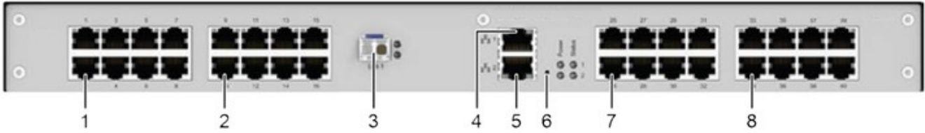
Figure 12. Front Panel, 32-Port Model with Grid Port and all CATx Ports
