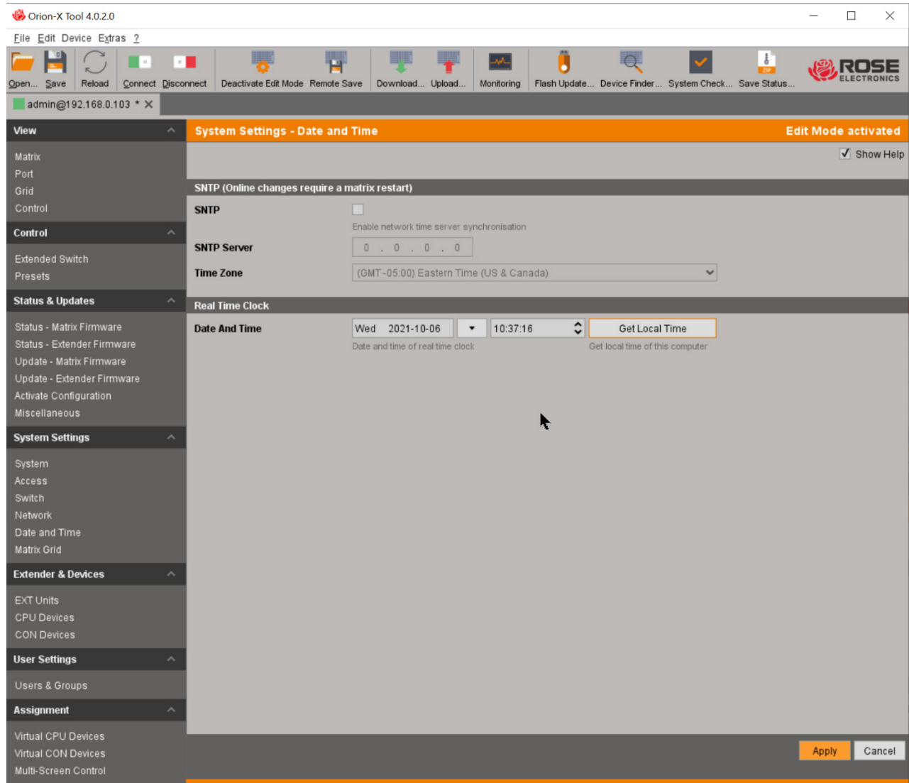
Figure 86. Modifying Date and Time Settings through the Java Tool
