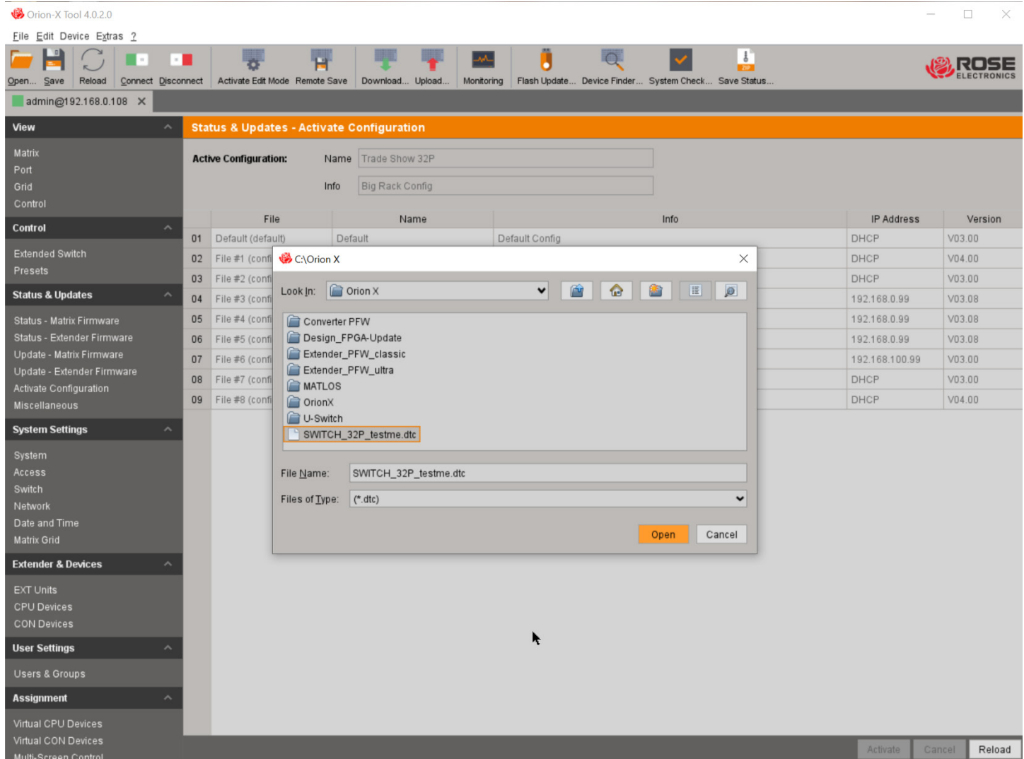
Figure 149. Loading external configuration through the Java Tool
