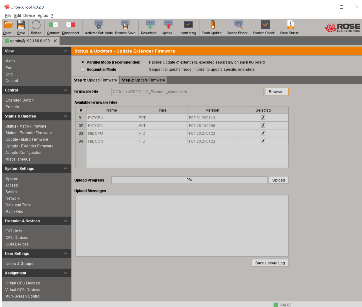
Figure 172. Extender Update in Standard Mode through the Java Tool - Step 1: Upload Firmware
