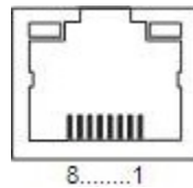
Figure 223. I/O Board RJ45 Connector
