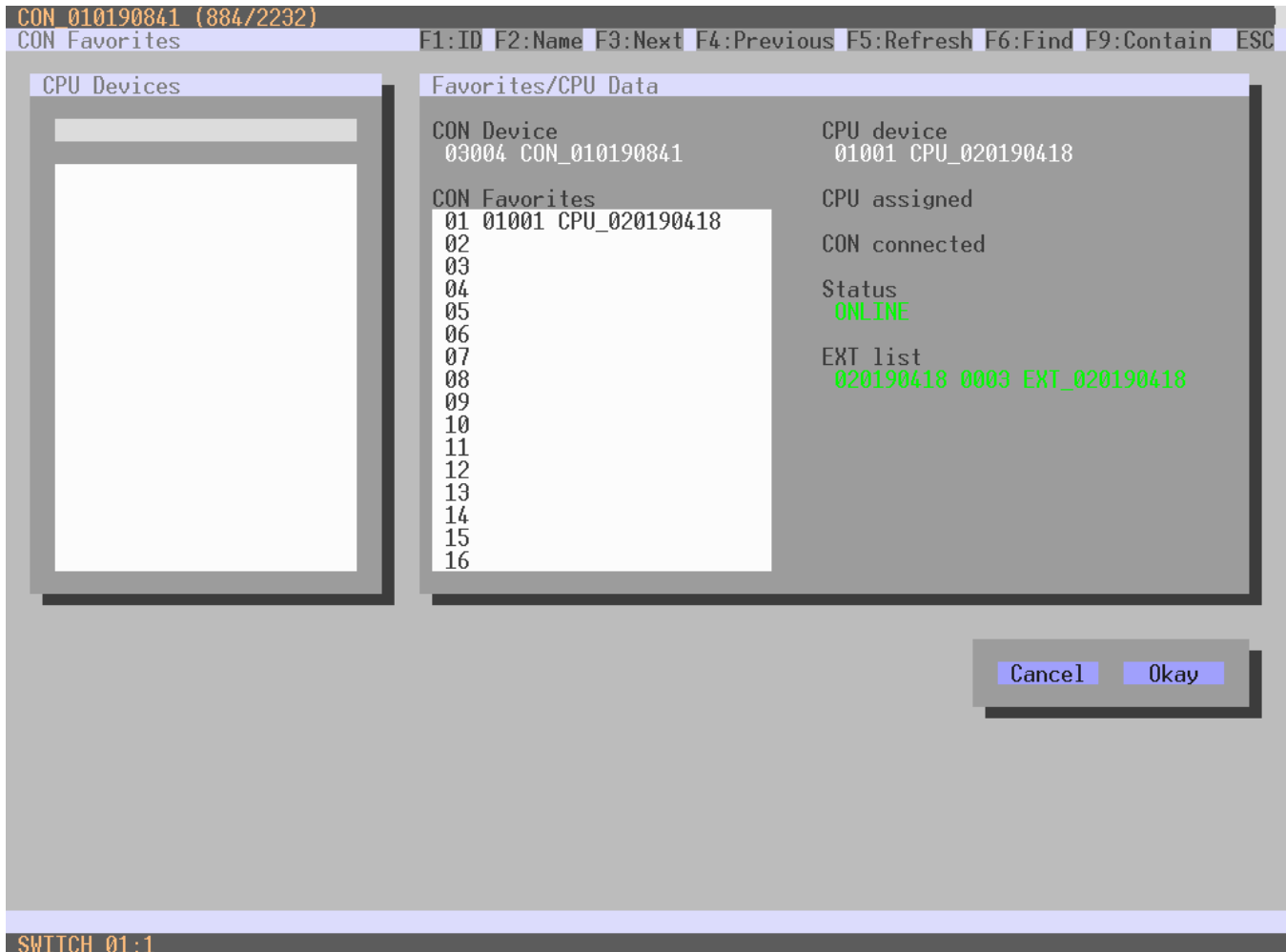
Figure 126. Setting up Console Favorites through the OSD
