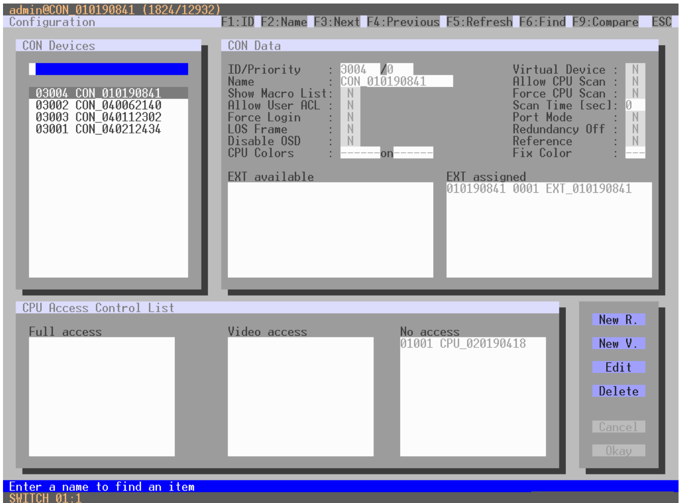
Figure 118. Setting Up CON Devices through the OSD
