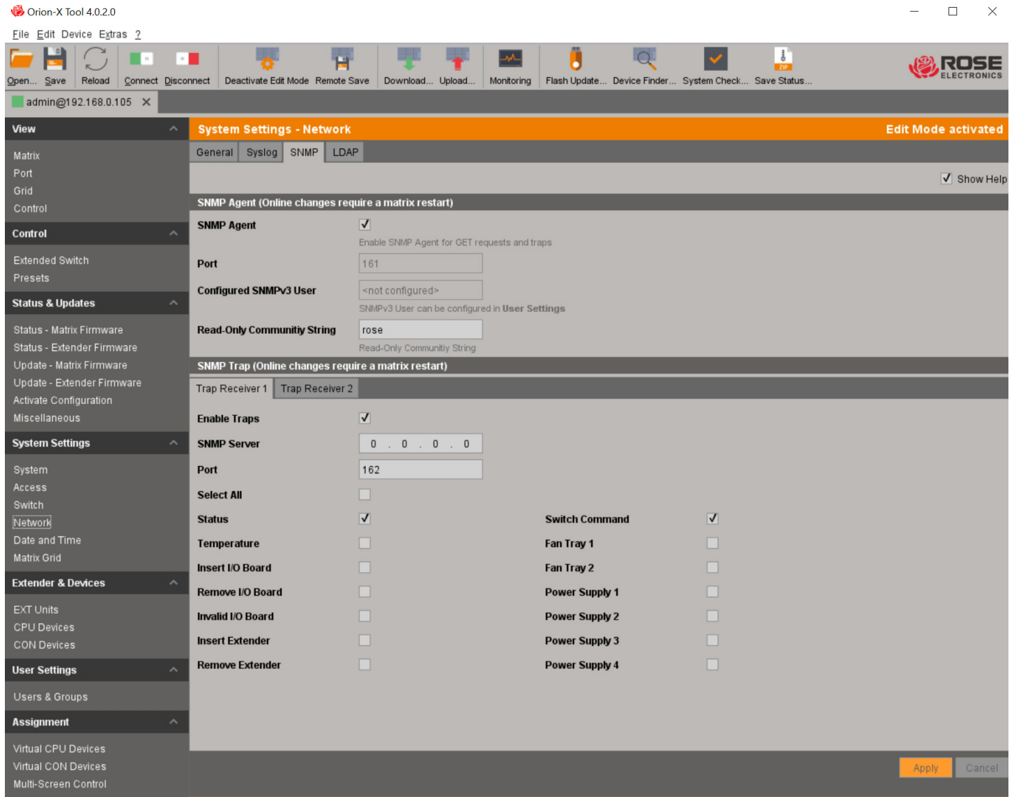
Figure 82. SNMP Monitoring through the Java Tool
