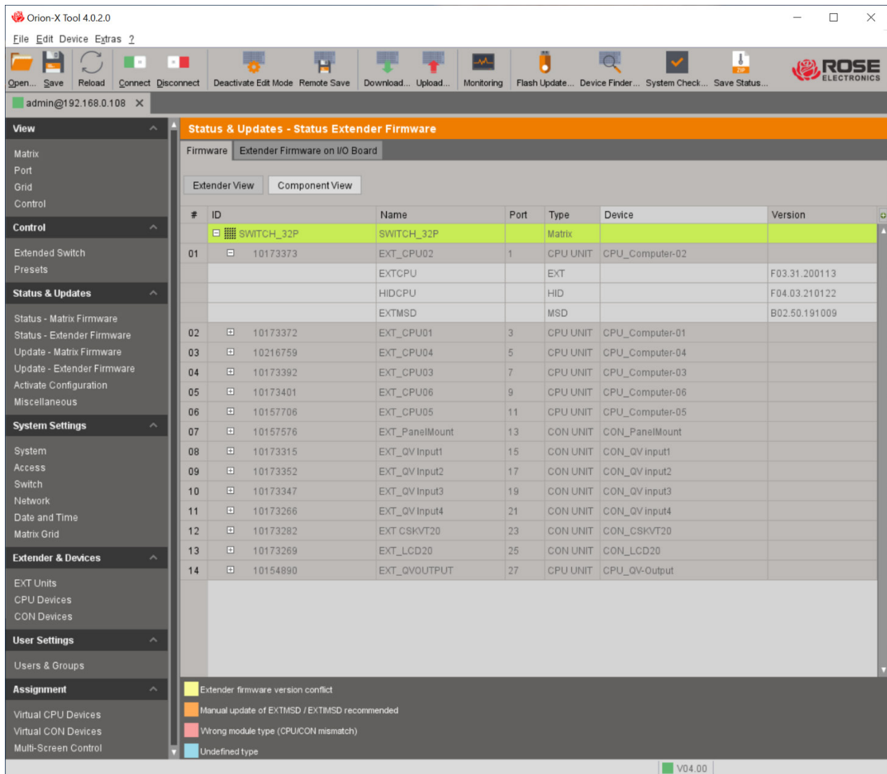
Figure 212. Expanded Firmware Status of Extender with the Java Tool
