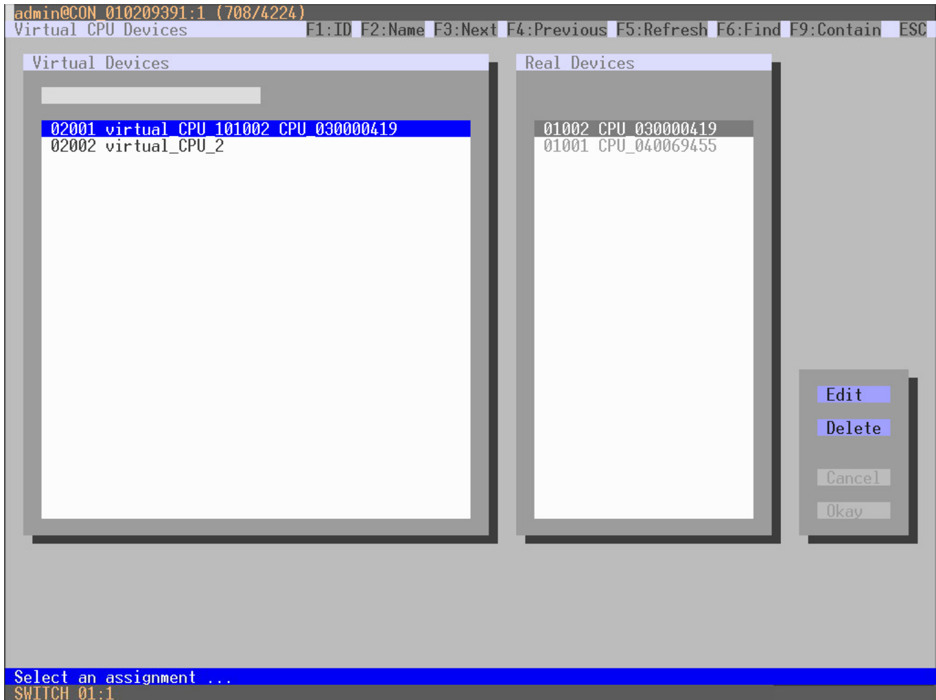
Figure 115. Virtual CPU Device Assignment through the OSD
