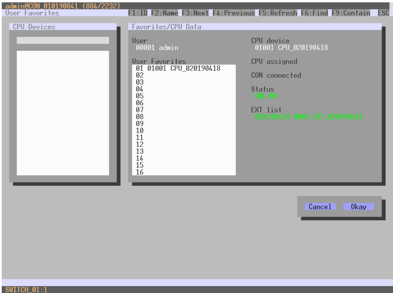
Figure 93. User Favorites OSD menu
