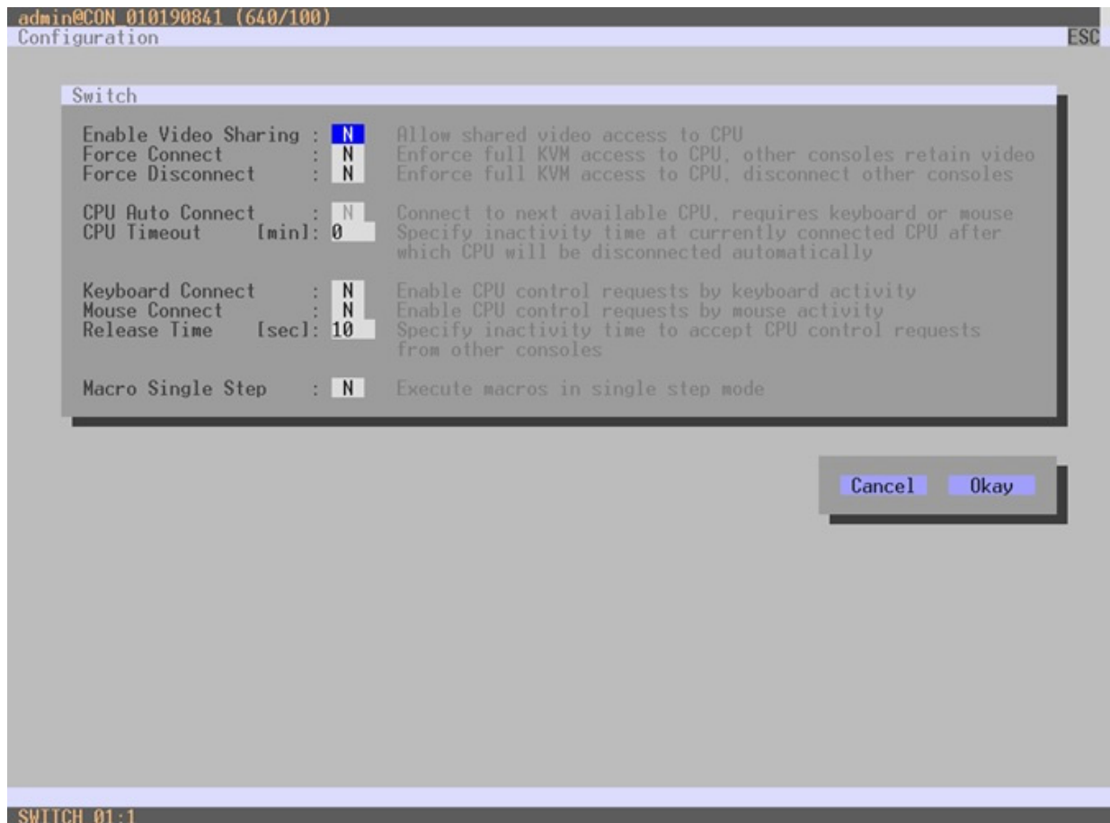
Figure 69. Modifying Switch Settings through the OSD
