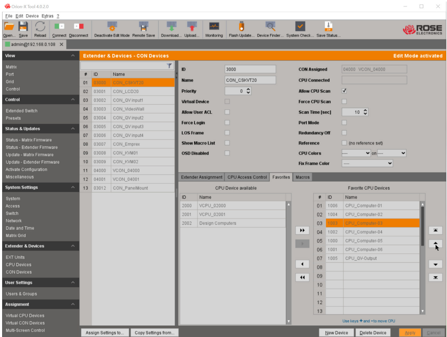
Figure 127. Setting Up Console Favorites through the Java Tool
