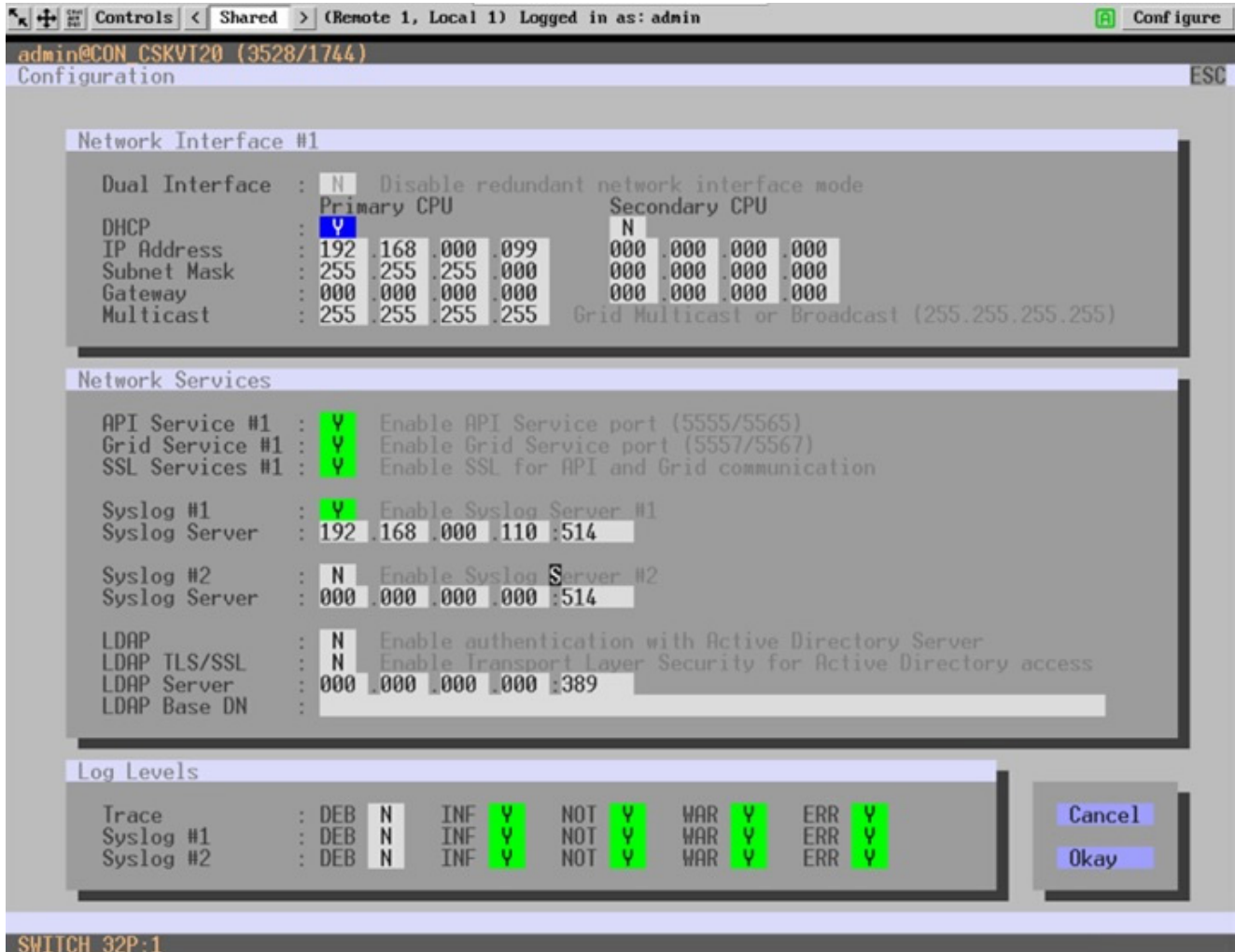
Figure 71. Modifying Network Settings through the OSD
