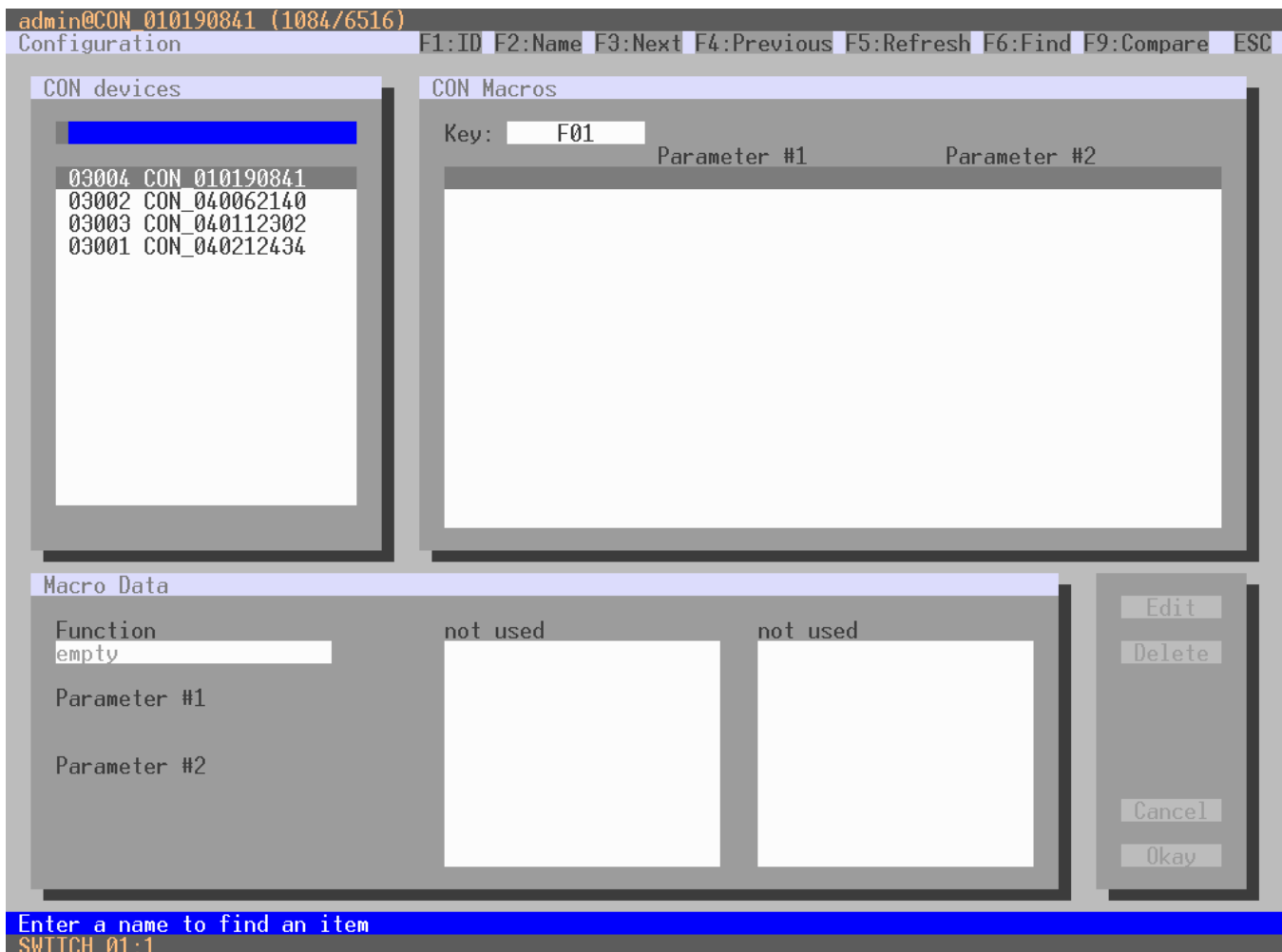
Figure 128. Setting Up Console Macros through the OSD
