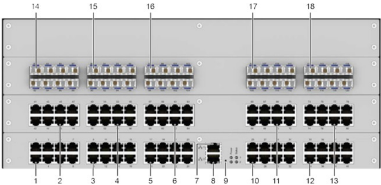
Figure 33. Front Panel, 120-Port Model with 80 CATx Ports and 40 Fiber Ports
