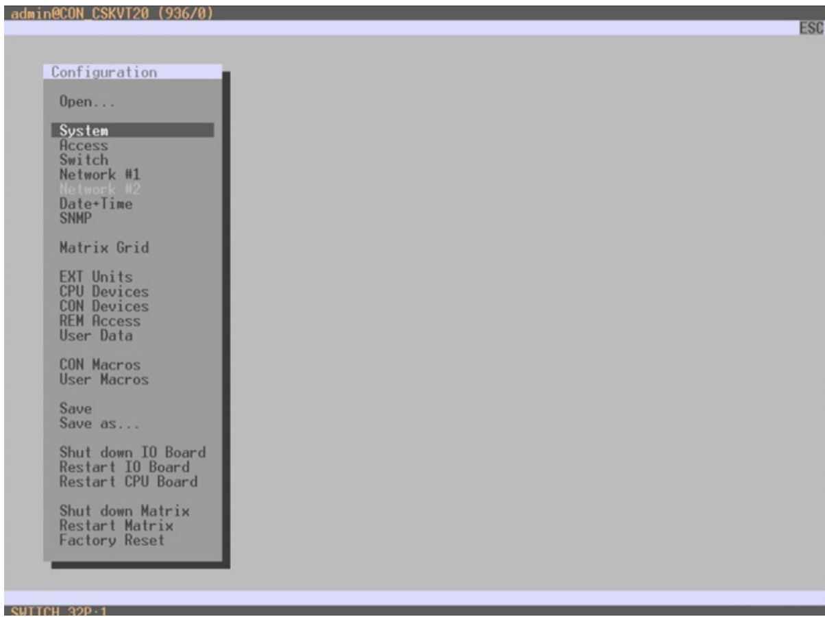
Figure 51. Configuration Menu in the OSD
