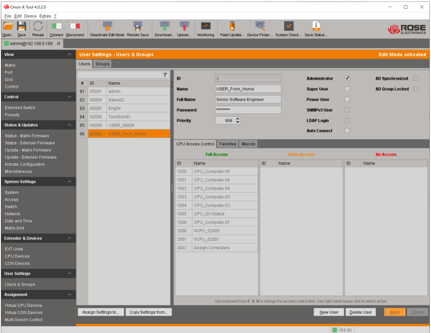
Figure 88. Modifying User Settings through the Java Tool
