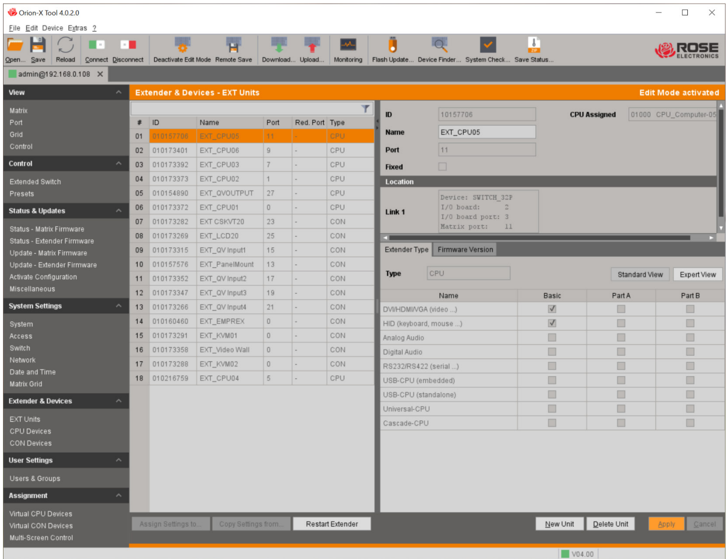
Figure 158. Setting Up Matrix Cascading Through the Java Tool
