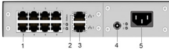
Figure 1. Front Panel, 8-Port Model with all CATx Ports
