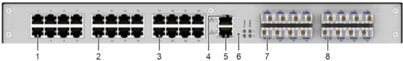
Figure 17. Front Panel, 40-Port Model with 24 CATx and 16 Fiber Ports
