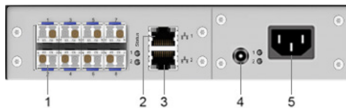
Figure 2. Front Panel, 8-Port Model with All Fiber Ports
