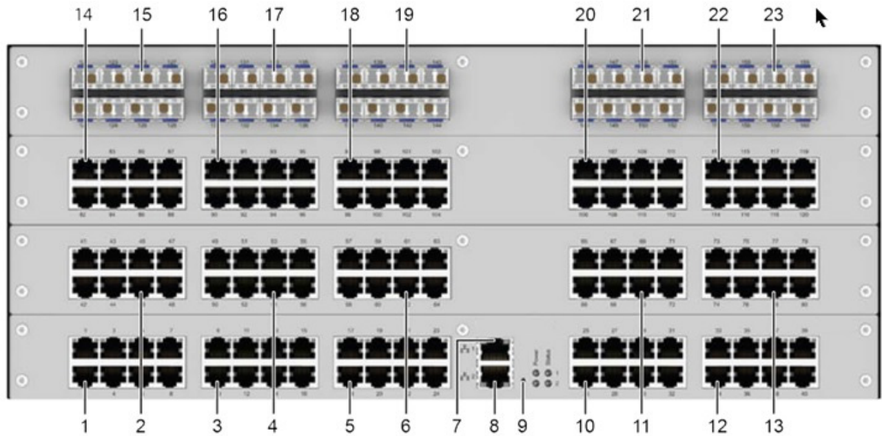
Figure 43. Front Panel, 160-Port Model with 120 CATx Ports and 40 Fiber Ports
