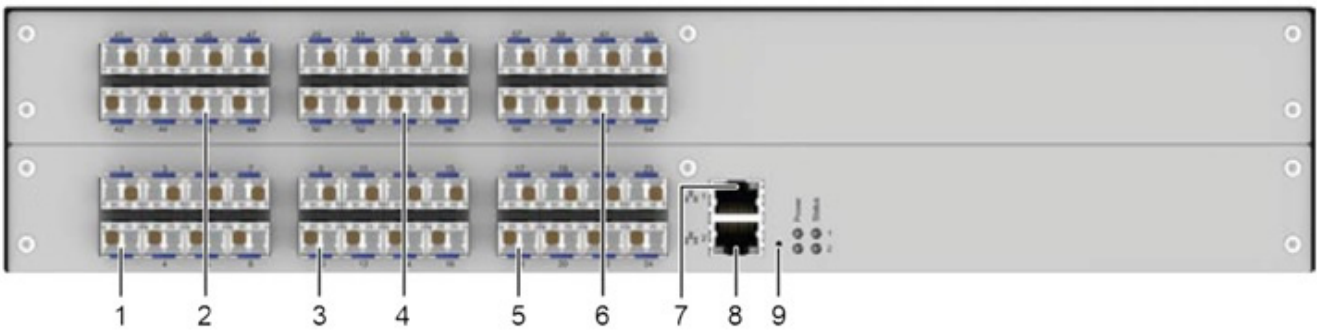
Figure 20. Front Panel, 48-Port Model with All Fiber Ports
