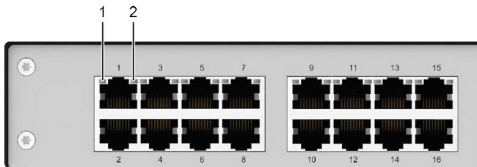
Figure 195. I/O Port Link Status Indicators, 1G CATx
