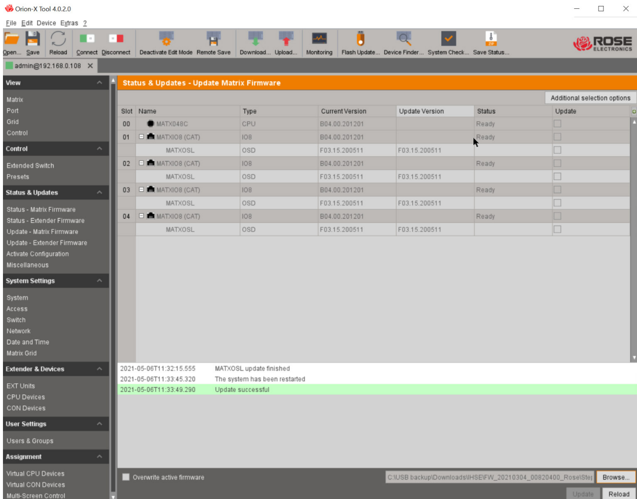
Figure 170. Firmware Update Success
