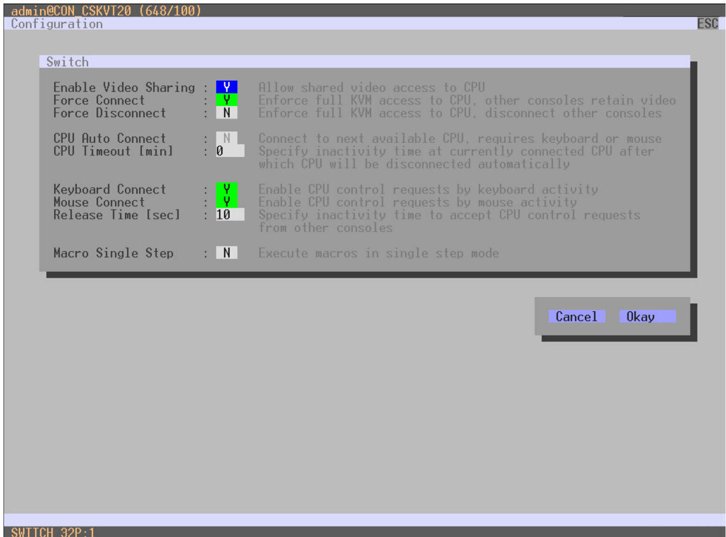
Figure 134. Enabling Shared Operation with the OSD
