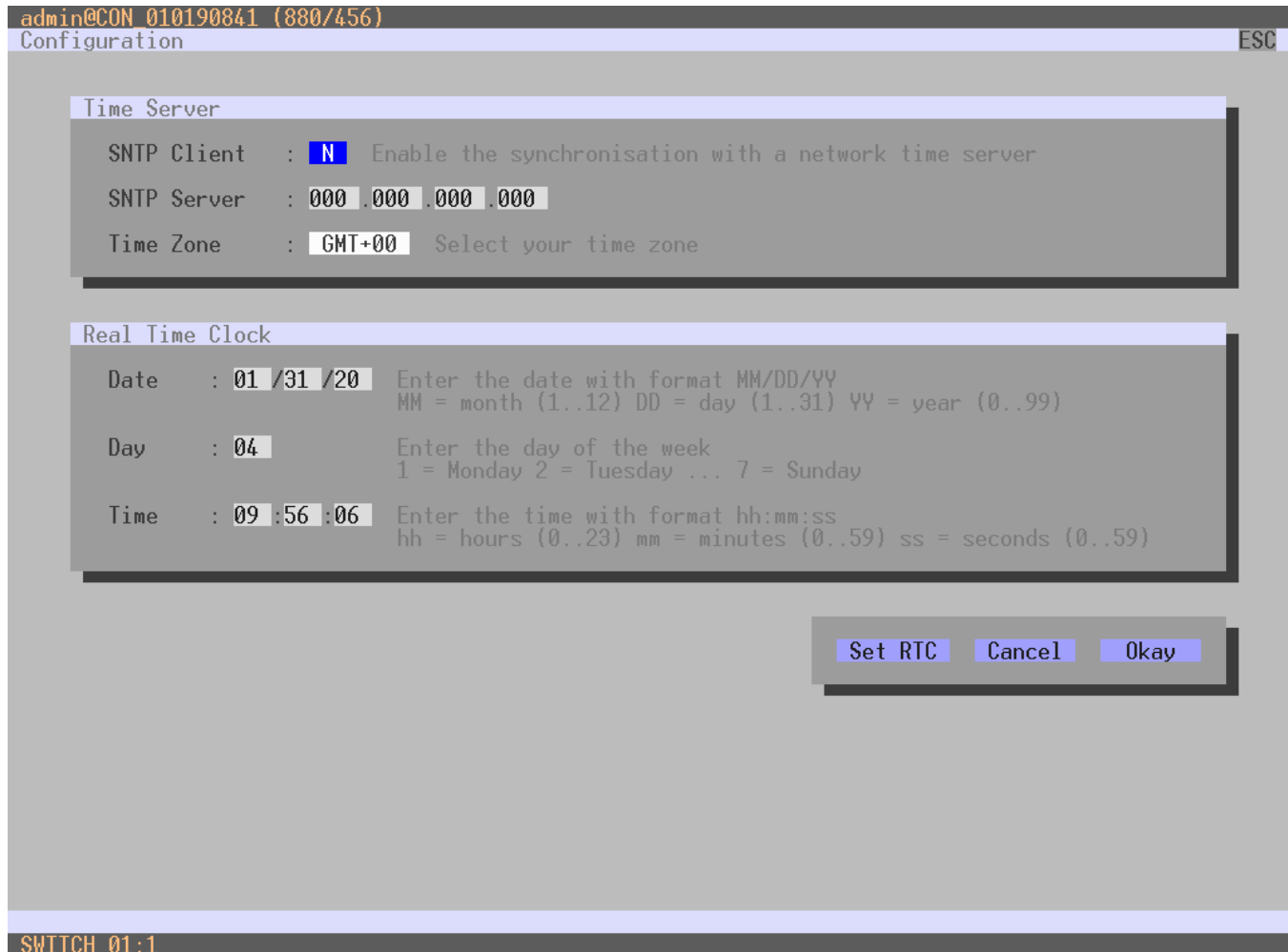
Figure 85. Modifying Date and Time Settings through the OSD
