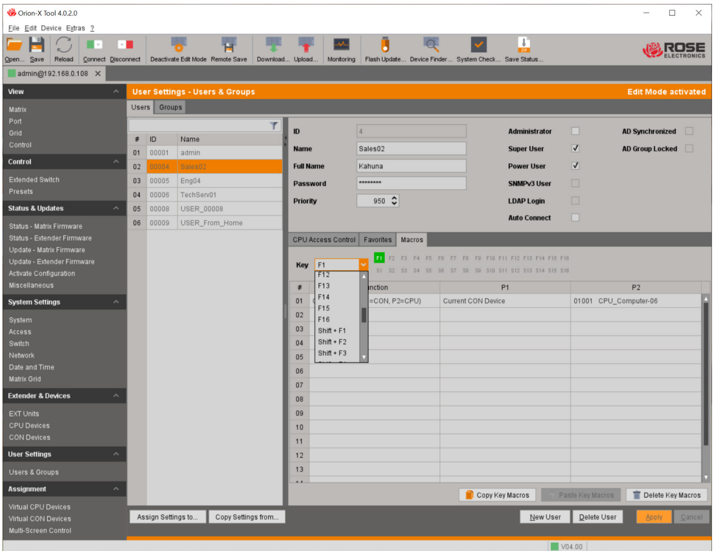
Figure 97. User Macros Function Key selection with Java Tool
