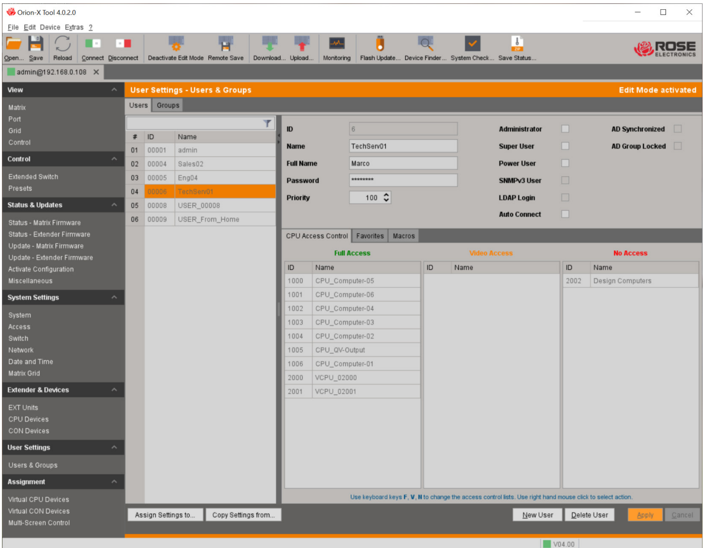
Figure 78. Creating a User for Active Directory with the Java Tool
